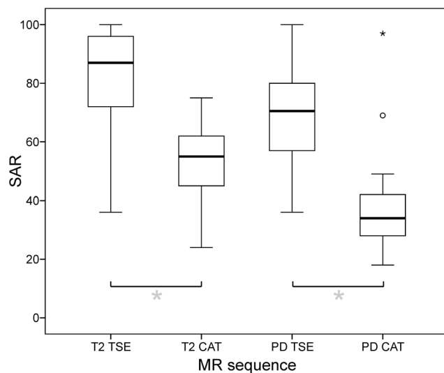
Figure 4. Specific absorption rate (SAR) of TSE and CAT sequences. Relative SAR reductions of CAT compared to TSE sequences was significant for both, the T2- ( 29.0 \pm 5.7\% ; p < 0.001 ) and the PD -contrast ( 32.7 \pm 21.8\% ; p < 0.001 ). (box: upper and lower quartiles, thick black line: median, whiskers: most extreme values of the interquartile range, circle: outlier, asterisk: extreme value; SAR values expressed as percentages of the effective SAR limit of 3.2 W/kg for head examinations according to IEC). doi:10.1371/journal.pone.0091030.g004
